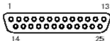
Fig.2-2 Pin Order of Parallel Port
